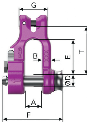
Pic. 27: ICE CCS-FASTLOX 4 mm
